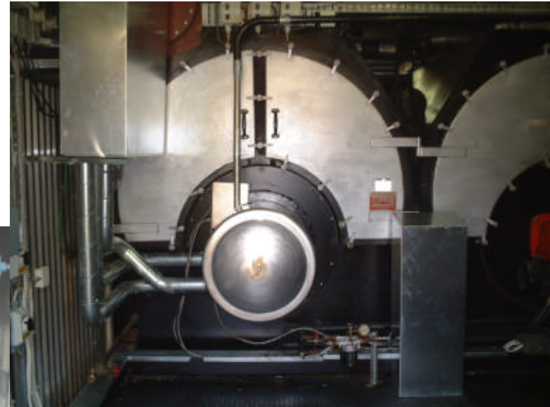
New burner, 500 kW th , in 25 yr old boiler
